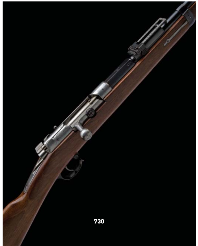
730 AN EXCEPTIONAL 11mm (COMMISSION) MAUSER M71/84 BOLT ACTION REPEATING SERVICE RIFLE SIGNED SPANDAU, serial no. 2804 , dated for 1888, with blued round 32in. barrel, block and blade fore-sight, elevating ladder rear-sight, 'SPANDAU' and crown markings to barrel near breech, rounded receiver in the white with model designation and date, straight bolt-handle, walnut full-stock with in the white heel-plate, blued furniture bar the bright stacking spike, light storage stains and marks but generally appearing in unissued condition and with all matching numbers £1,000-1,500
